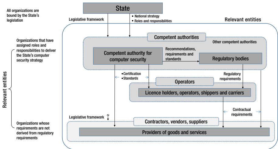
FIG. 5. Organizations having computer security responsibilities within a nuclear security regime.
