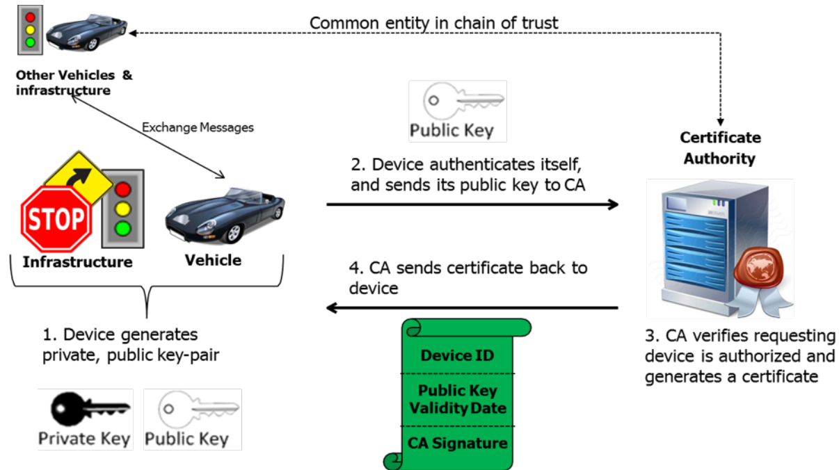
Figure 4 – V2X Public Key Infrastructure Overview [9]
