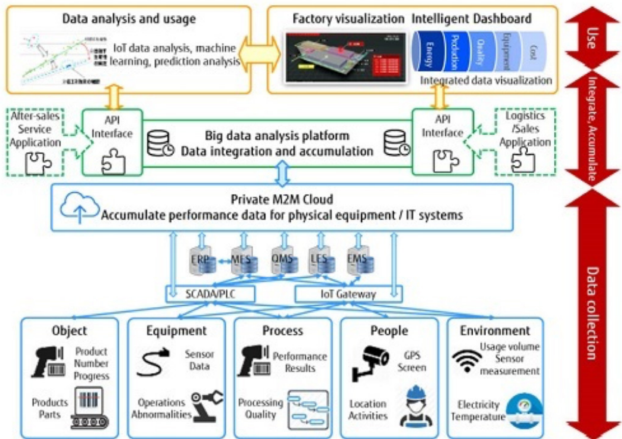
Figure 9 – An Example of a Smart Manufacturing Environment
